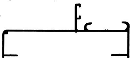
ALG 195 Marco puerta 25mm 0.490 kg/m
