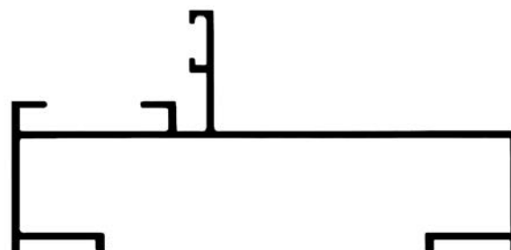
ALG N11 Marco puerta 25mm 0.650 kg/m
