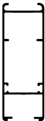
ALG 413 Parante puerta 25mm 0.670 kg/m
