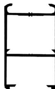
ALG N12 Parante puerta 25mm 0.460 kg/m
