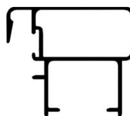
ALG N4/L Parante central ventana corrediza 0.390 kg/m
