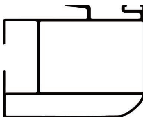
ALG 035 Parante central corrediza 1.531 kg/m
