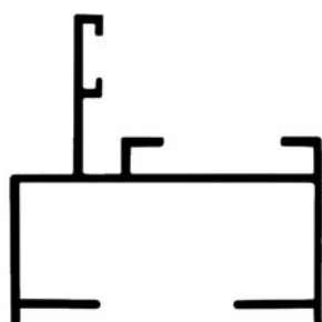
ALG N10 Marco puerta 25mm 0.400 kg/m
