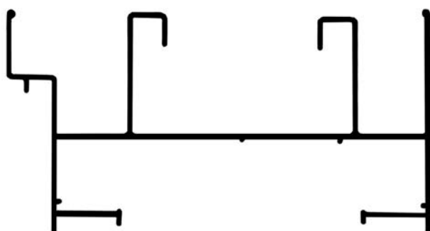
ALG N1/P Marco ventana corrediza 0.650 kg/m
